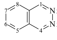
Phtalazine
