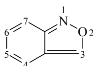
Anthranil
