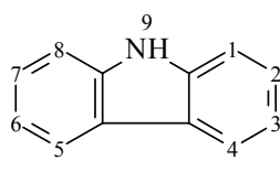
Carbazole
