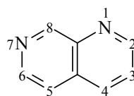
Pyrido[3,4-b]pyridine
