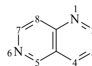
Pyrido[4,3-b]pyridine
