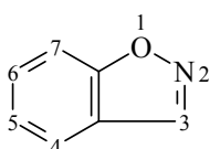
Indoxazine
