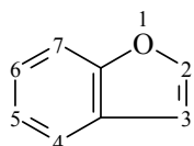
Coumarone
