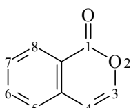
Isocoumarine
