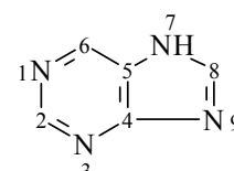
Purine
