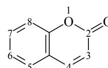
Coumarine
