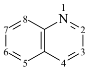
Quinololine
