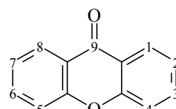
Xanthone
