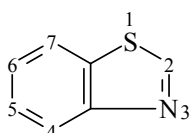
Benzothiazole
