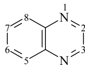
Quinoxaline
