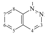
Cinnoline
